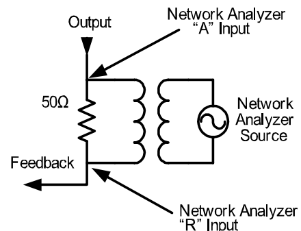
Figure 7. Transformer Injection
